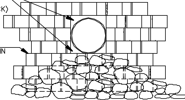
LARGE PIPE THROUGH STONEWALL (FRONT VIEW)
