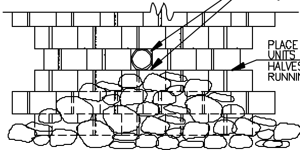
SMALL PIPE THROUGH STONEWALL (FRONT VIEW)
